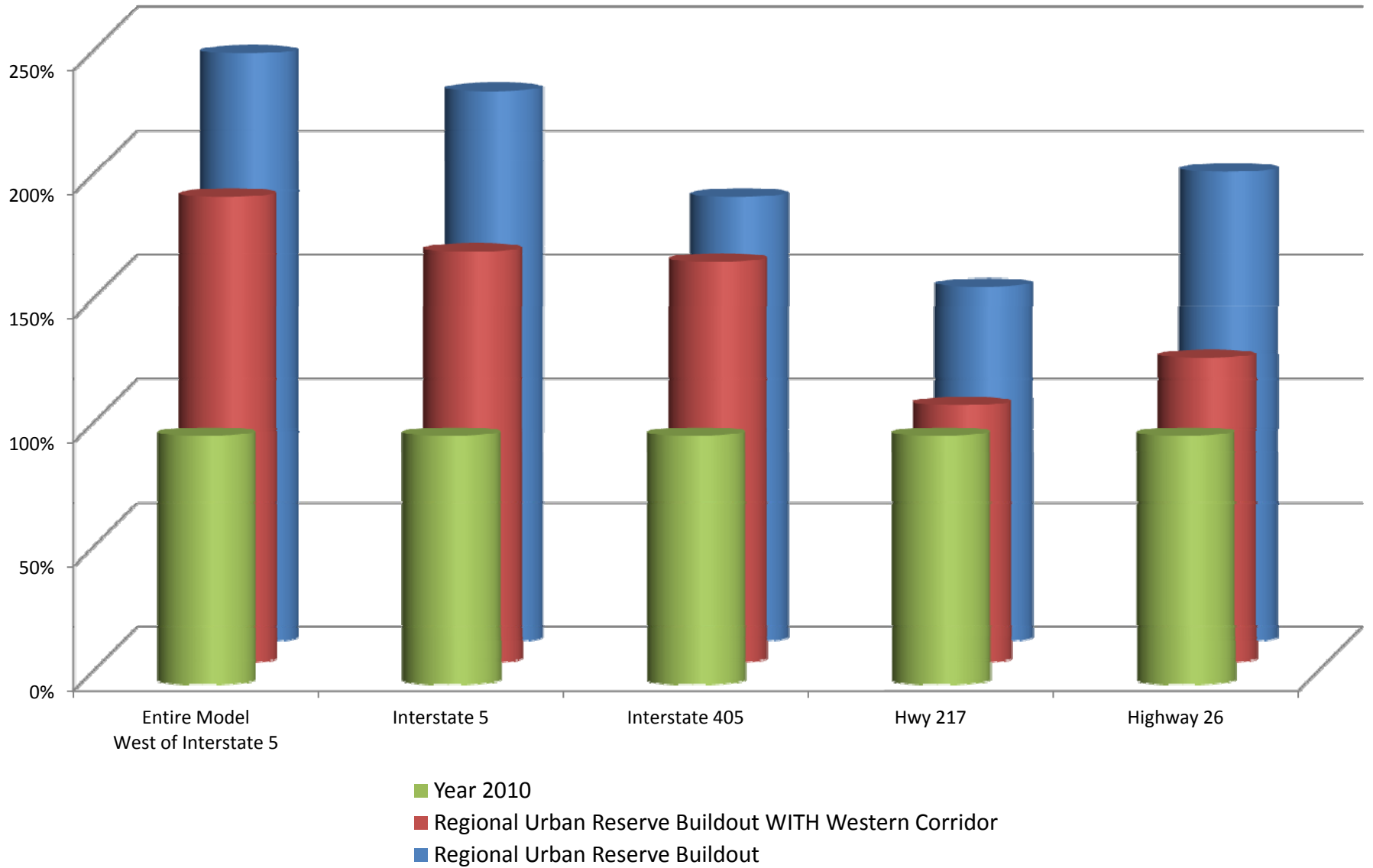
Chart 3A: Percent Increase of Vehicle Hours of Delay Relative to Year 2010 Limited Access Facilities (PM Peak Two-Hour)
